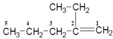
2-Ethyl-1-pentene
