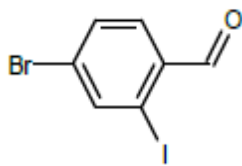
2-bromo-4-iodobenzaldehyde
