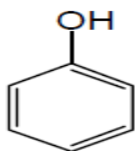
Phenol
