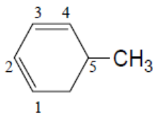
5-Methyl-1,3-cyclohexadiene
