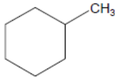
Methyl cyclohexane
