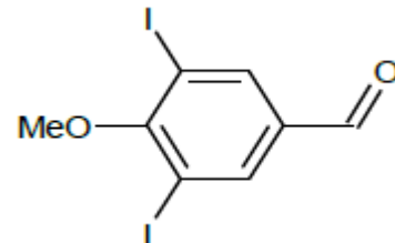
3,5-diiodo-4-methoxy Benzaldehyde
