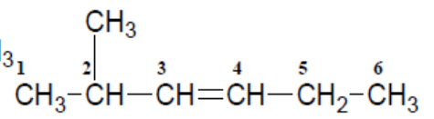
2-Methyl-3-hexene
