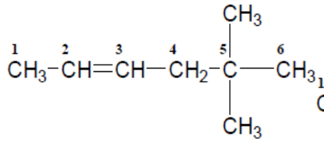
5,5-Dimethyl-2-hexene
