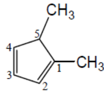
1,5-Dimethyl-1,3-cyclopentadiene
