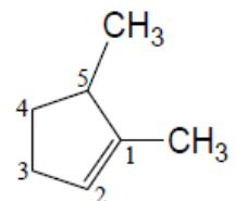
1,5-Dimethyl cyclopentene
